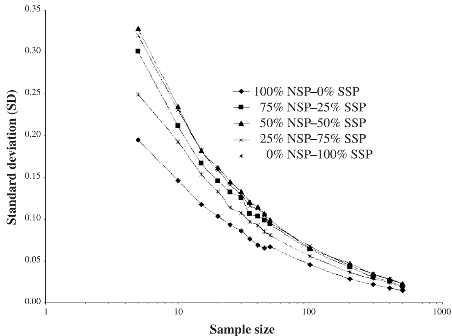
Fig. 3. Standard deviation (SD) plotted against sample size used in the calculation of the mixed stock analysis. The standard deviation for each sample size-treatment is evaluated from 1000 bootstraps taken from a known population admixture (five different compositions).
