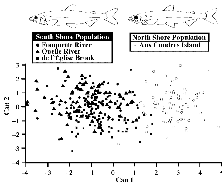
Fig. 7. Distribution of adult smelt sampled in 1998 as a function of the two principal canonical axes. Discriminant analysis was performed using 16 morphometric measurements (corrected for size effect through a principal component analysis) and two meristic counts. The grouping variable used for discriminant analysis was the sampling site. Open circles represent fish from Aux Coudres Island (NSP); filled circles, Fouquette River (SSP); filled triangles, Ouelle River (SSP); filled squares, de l'Église Brook (SSP).
