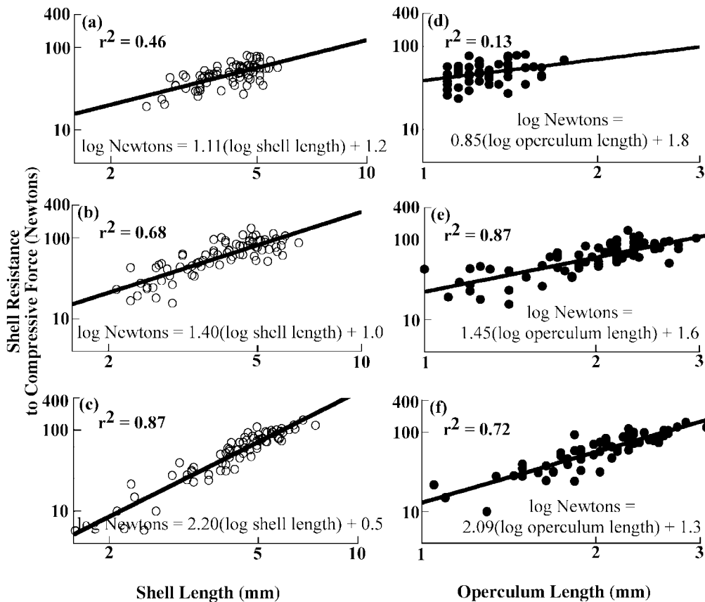
Fig. 5. Shell resistance to crushing versus shell length (a, b, c) and operculum length (d, e, f). The force needed to crush (a) Mexipyrus carranzae ( P < 0.001 ), (b) Mexithauma quadripaludium ( P < 0.001 ) and (c) Nymphophilus minckleyi ( P < 0.001 ) increased significantly for all three species of snails as their shell length increased. We used Mexithauma quadripaludium in experimentally estimating crushing performance.
