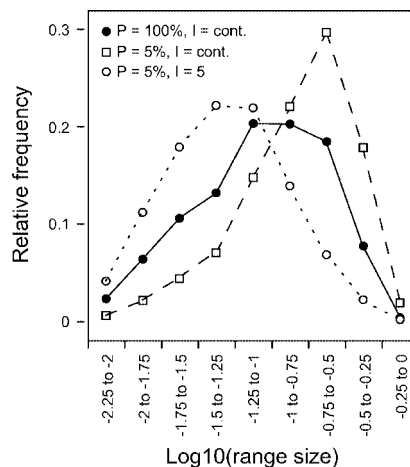
Fig. 4. A graphical representation of the relative range size frequency distributions for different combinations of sub-sample partiality (P) and isolate number (I). Closed circles represent the relative proportions of species whose log latitudinal ranges fall within each bin when sub-sampling is comprehensive (P = 100%) and isolates are continuous (I = cont.). Squares represent the relative proportions of species whose log latitudinal ranges fall within each bin when sub-sampling is highly partial (P = 5%) and isolates are continuous (I = cont.). Finally, open circles encompass the situation when partiality is high (P = 5%) and number of isolates is low (I = 5).
