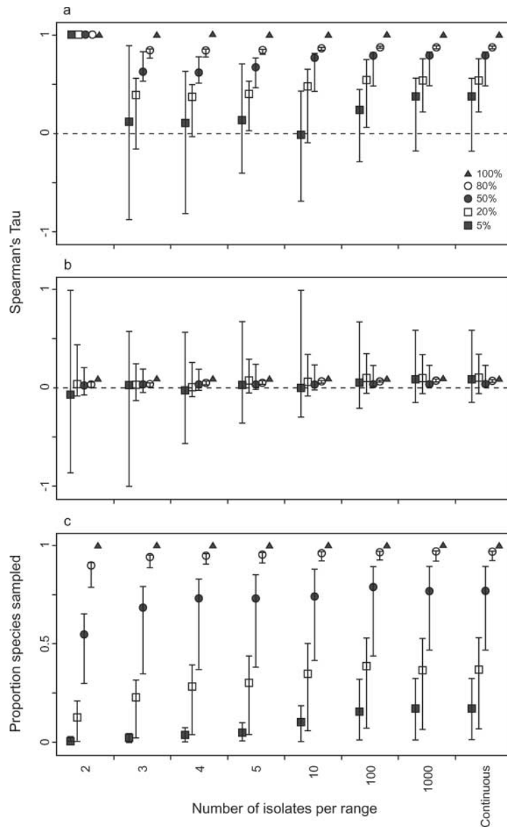
Fig. 2. A graphical representation of the weakening relationship between range size and body size for New World mammals as a function of sampling partiality and number of isolates within a given species range. Panel (a) shows the analysis when assuming that body size is equal to range size – representing a strong underlying relationship. Panel (b) shows the analysis when real mammal body size estimates are used – representing a weak underlying relationship. Presented are the medians for five different degrees of sampling partiality (5, 20, 50, 80 and 100%) and the corresponding 95% confidence ranges – a measure of the statistical uncertainty for each realization of a given sample. The number of isolates (the x-axis) ranged from two, where only the endpoints of a species range were considered, through to continuous over a species range. Panel (c) shows the median proportion of the total species intercepted by a sub-sample for each combination of isolate number and sampling partiality and the corresponding 95% confidence ranges.
