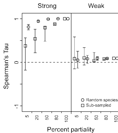
Fig. 3. A graphical representation of the difference between the estimated correlation coefficients and 95% confidence ranges under the sub-sampling regime shown in Fig. 2 (open squares) and a random sub-sampling regime (open circles). Simulations were run using both a strong (left-hand side of the graph) and a weak (right-hand side of the graph) underlying relationship. Isolates were continuous and all levels of partiality were examined.
