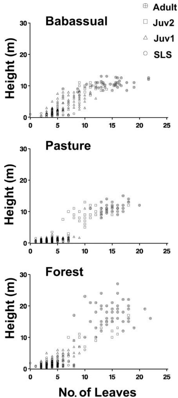
Fig. 2. Number of leaves plotted against total height. A different symbol is used for each stage. Entire-leafed seedlings are not plotted because they are too numerous and all occupy roughly the same position in the number of leaves–height plane. Sometimes, all leaves of a palm tree have been cut or damaged, which results in individuals with a height and no leaf.
