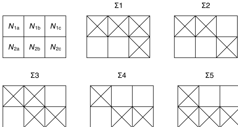
Fig. 4. Solution types ( \Sigma 1 through \Sigma 5 ) for a system with two bee species and three flower types. A crossed square indicates that N_{ij} > 0 (with i, j as in the top-left drawing).
