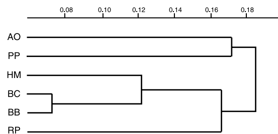
Fig. 1. Phylogenetic hypothesis depicting relationships between the six species on the basis of genetic distances for three genes: 12S, 16S, and cyt b . AO = Alytes obstetricans , PP = Pelodytes punctatus , BB = Bufo bufo , BC = Bufo calamita , HM = Hyla meridionalis , RP = Rana perezi .
