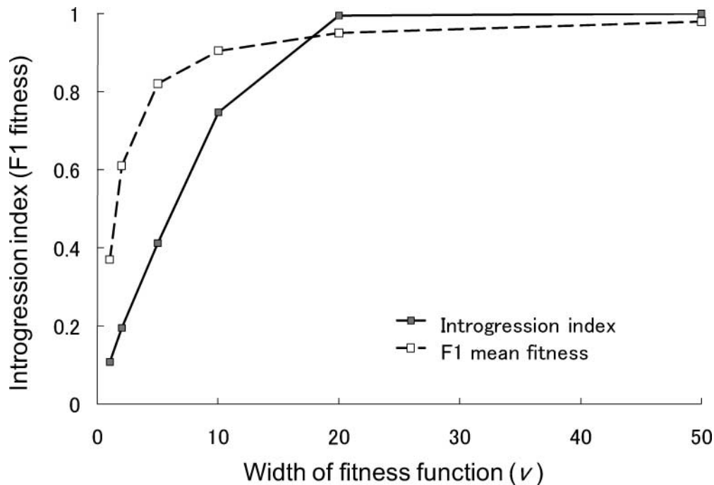
Fig. 5. Asymptotic introgression index plotted against the measure of directional selection (width of fitness function). The fitness function is the local adaptation model. The total number of simulated generations is 200. Other parameter values are n = 10 , R = 0.2 , and m = 0.05 .
