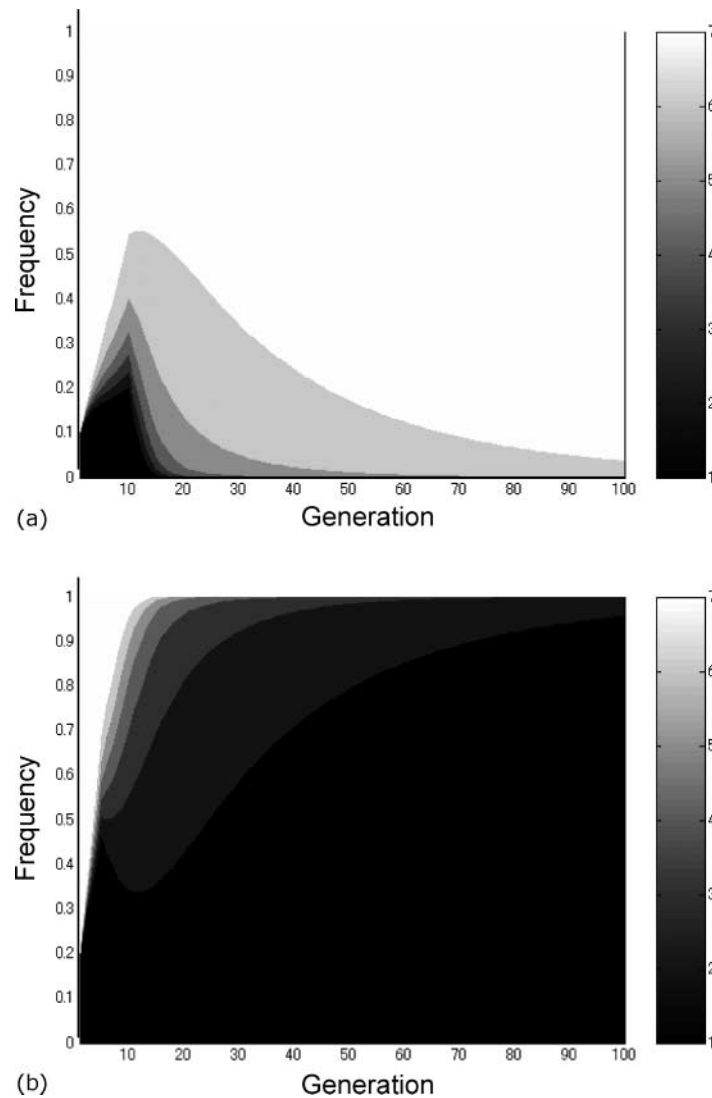
Fig. 9. Simulated introgressive hybridization by pulse invasion that is (a) low-rate and long-term ( m = 0.1, T = 10 ) and (b) high-rate and short-term ( m = 0.2, T = 5 ). The y-axis represents gamete class frequencies. There are 11 gamete classes and 10 loci: the black class (1) is the purely exotic gamete, and the white class (11) is the purely endemic gamete. Other parameter values are n = 6 and R = 0.4 .
