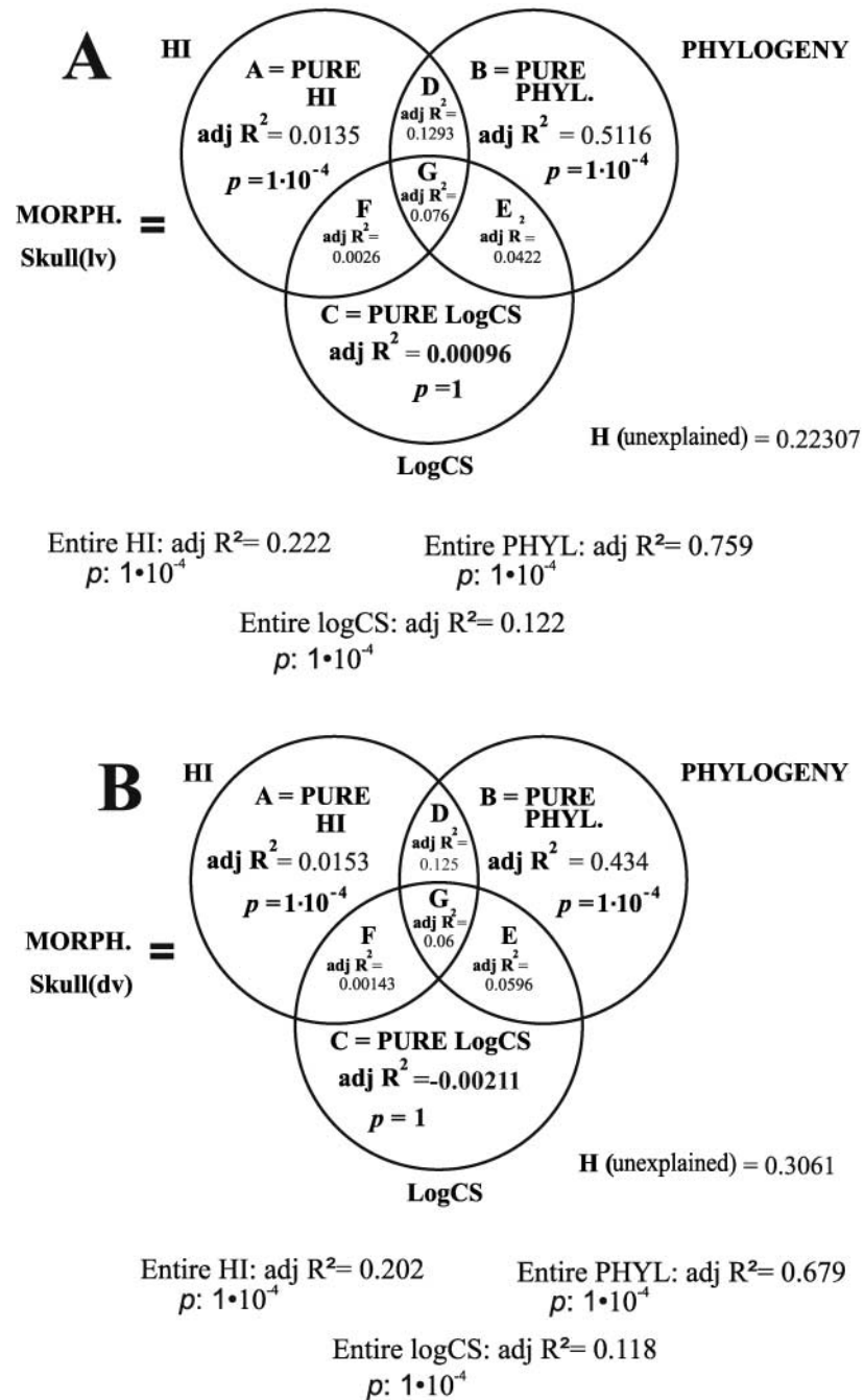
Fig. 7. VARPART results for the four configurations.
