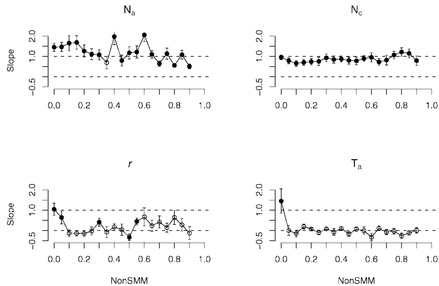
Fig. 4. Slope comparing the actual N_a , N_c , r or T_a with the modes of the posterior distributions from models including the true value, Geweke, and ESS -1 . The slopes as well as standard errors are given. Slopes significantly different from 0 represented by solid circles while slopes not significantly different from zero represented by open circles.
