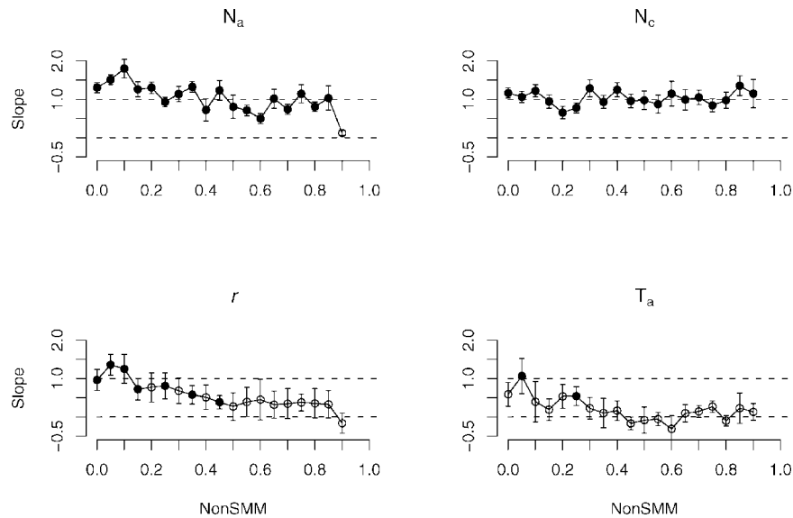
Fig. 5. Analyses of N_a , N_c , r and T_a in UGM. The slope comparing the actual N_a , N_c , r or T_a with the modes of the posterior distributions from models including the true value, Geweke, and ESS^{-1} . The slopes as well as standard errors are given. Slopes significantly different from 0 represented by solid circles while slopes not significantly different from zero represented by open circles.
