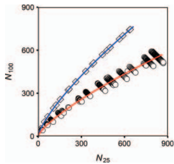
Fig. 3. Expected IFD and MAXN isodars (linear scale) for Folsomia candida choosing between high- versus moderately-low-quality (100% vs. 25%) habitats. IFD (diamonds) and MAXN (circles) isodar solutions based on all possible comparisons of density ( N ) at 20 different population sizes. Blue and red lines correspond with solutions (from Fig. 1) to equations (4, IFD) and (5, MAXN) respectively.
